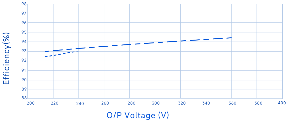
Efficiency Vs. O/P Voltage (Vin=120Vac)
